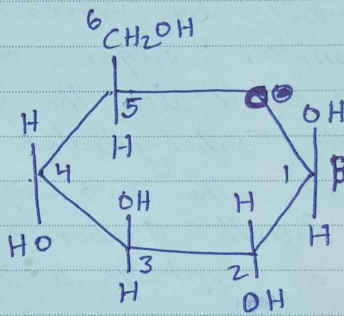
\beta D = Glucose
